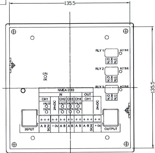
REAR ELEVATION (PANEL MOUNTS AND CONNECTORS NOT SHOWN)
