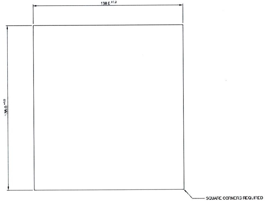
REAR ELEVATION (PANEL MOUNTS AND CONNECTORS NOT SHOWN)
